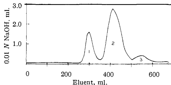
Fig. 1.—Chromatogram of levopimaric acid isomerized for three hours at 155°; peak 1, palustric acid; peak 2, levopimaric and l -abietic acids; peak 3, neoabietic acid.
